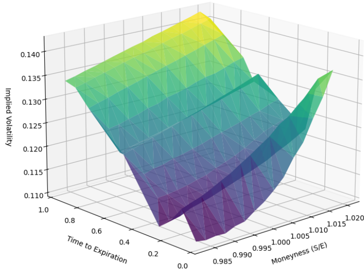
Figure 2: Implied Volatility Surface.
